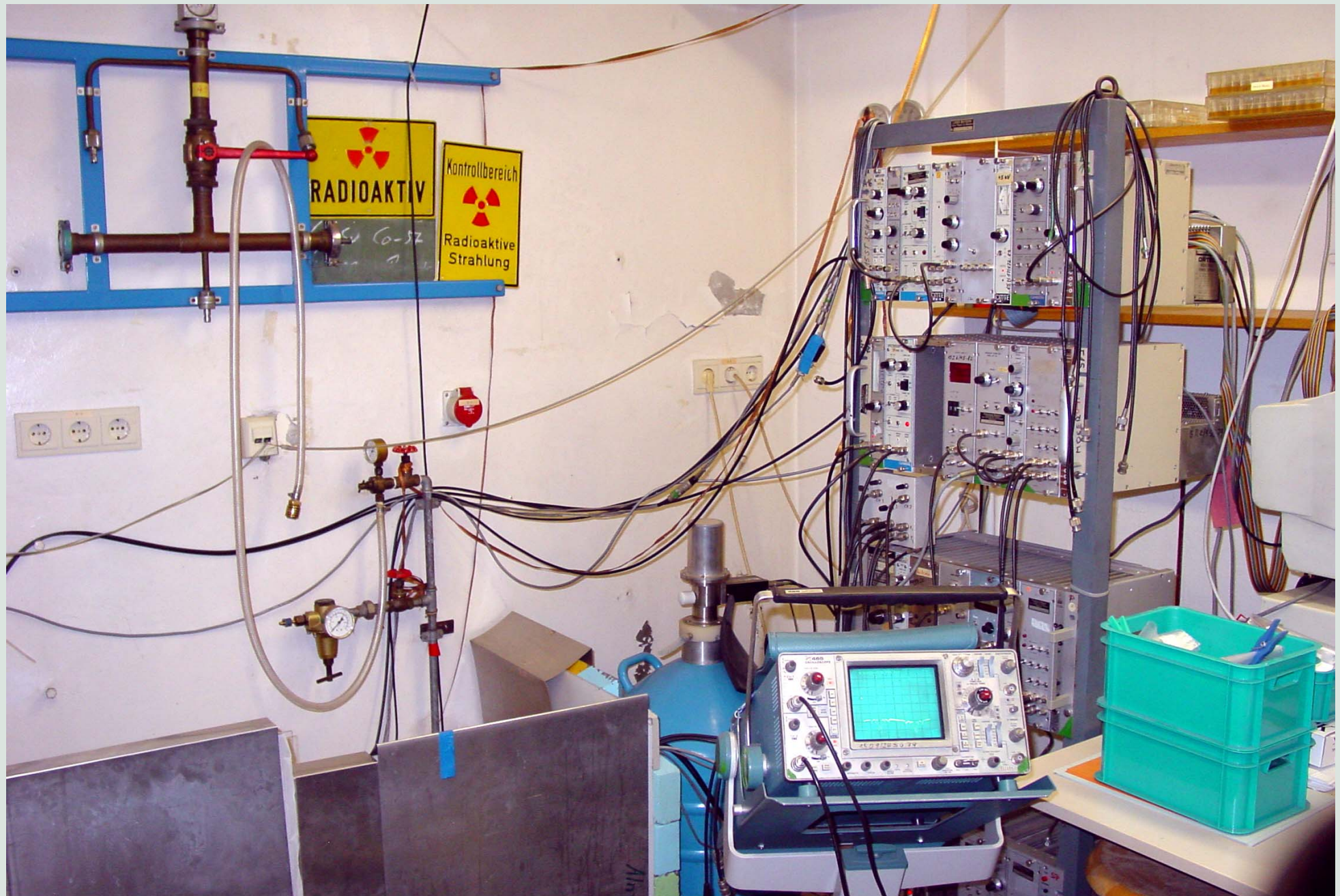
Mössbauer measurements at RT: behind the black shielding are three spectrometers
